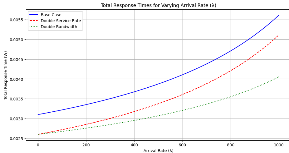
Fig.4. Total response time (W) with varying arrival rates for M/M/c model
