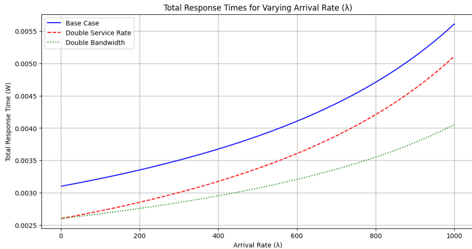
Fig. 5. Total response time ( W ) with varying arrival rates, base case, double service rate and double bandwidth scenario ( \mu = 1000 , \mu_{ES} = 10000 , c = 10 , \delta = 0.5 , \mu_{DS} = 1000 , \mu_{OS} = 2000 )
