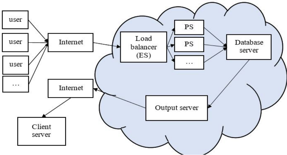
Fig.1. queuing theory model in cloud computing
