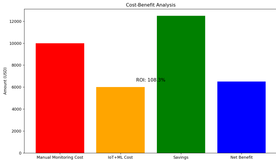
Fig. 10. Cost–Benefit Analysis.
