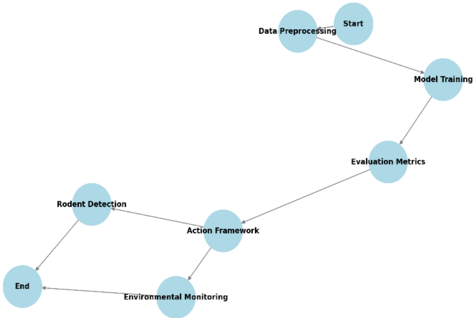
Fig.1. Overall Workflow.
