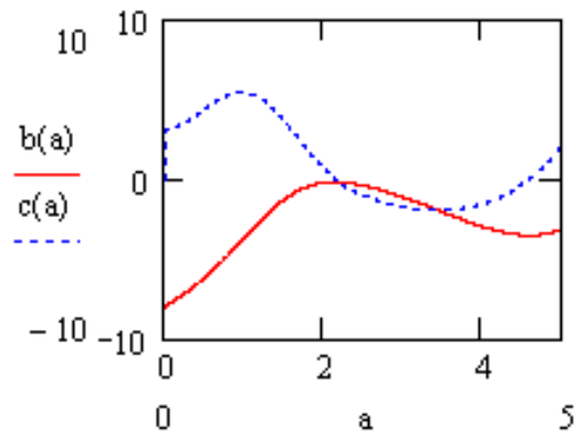
Fig. 2. The graph of the solution of a given differential equation b(a) and the derivative of the solution function – c(a)
